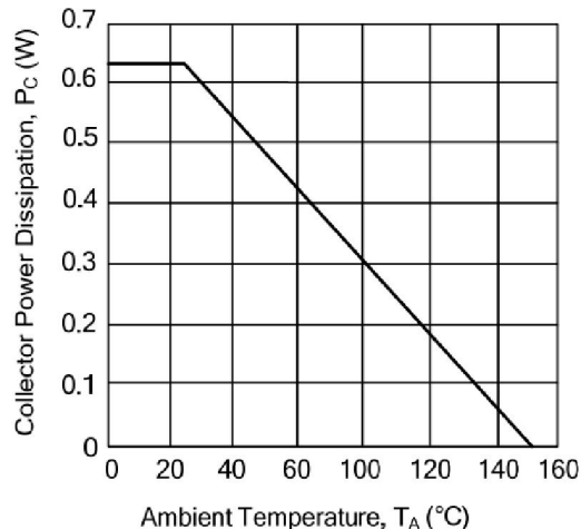
Figure 6. Power Derating
