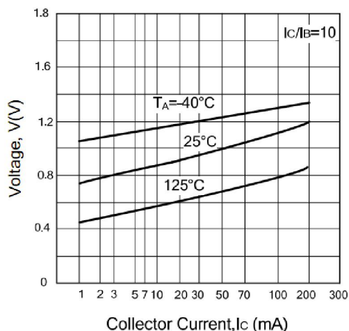
Figure 3. Base-Emitter Voltage
