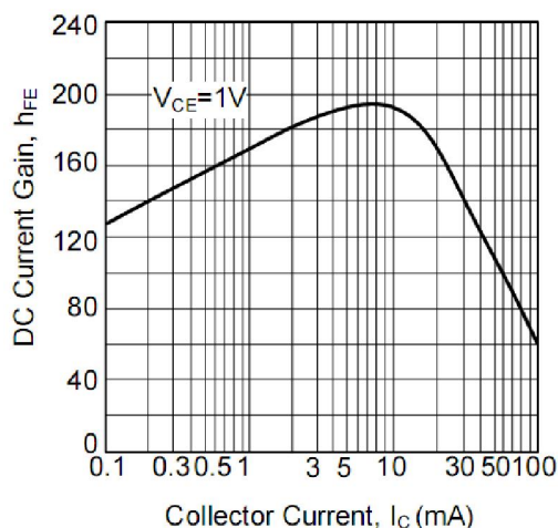
Figure 1. DC current Gain
