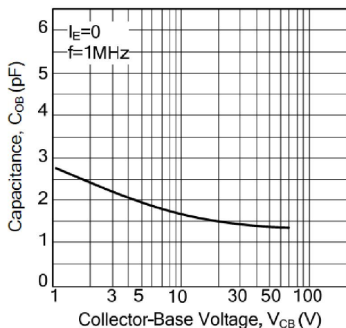
Figure 5. Collector Output Capacitance
