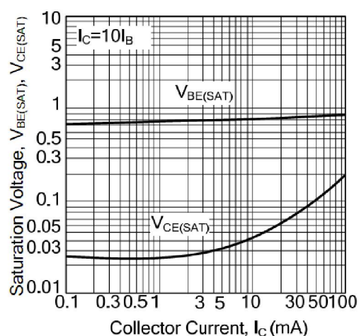
Figure 2. Saturation Voltage
