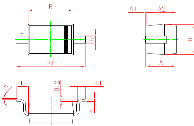
SOD-323
