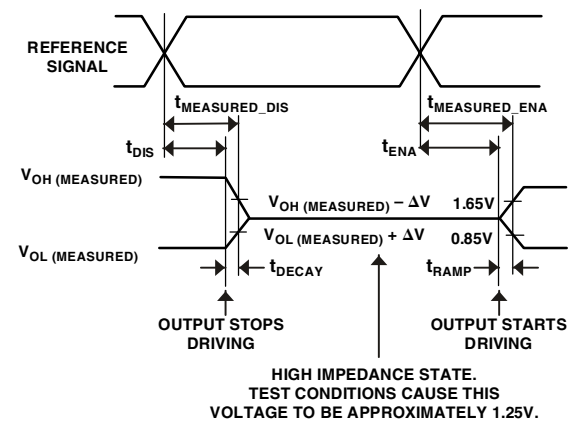
Figure 35. Output Enable/Disable
