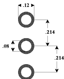
TO-247-3
