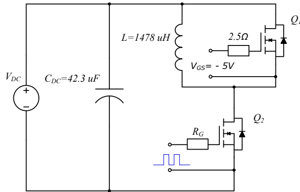
Figure 29. Clamped Inductive Switching Waveform Test Circuit
