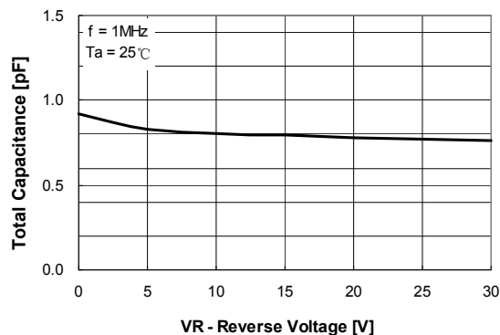
Figure 2. Total Capacitance
